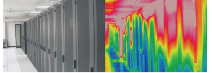
Fig. 7. The thermal image of an aisle in a data center. The infrared thermal image shows significant variations on intake air temperature across racks and at different height [18].
